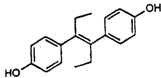
Diethylstilbestrol
